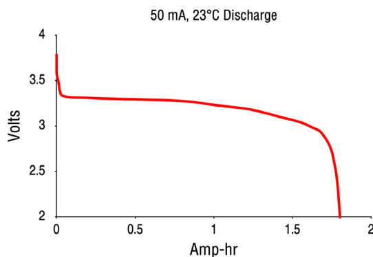
Discharge Curve 50 mA, 23°C
