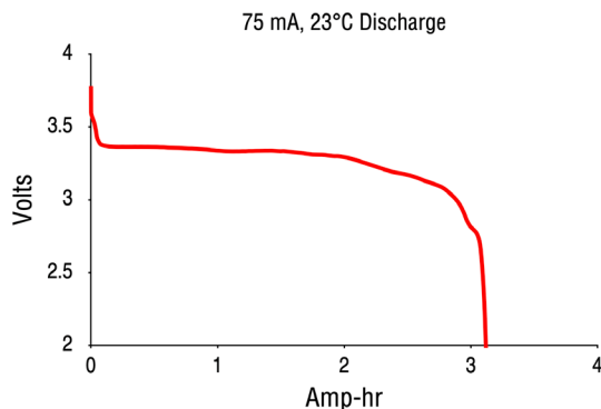
Discharge Curve 75 mA, 23°C
