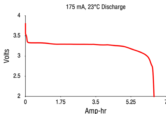
Discharge Curve 175 mA, 23°C
