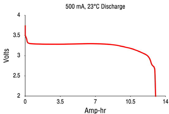
Discharge Curve 500 mA, 23°C
