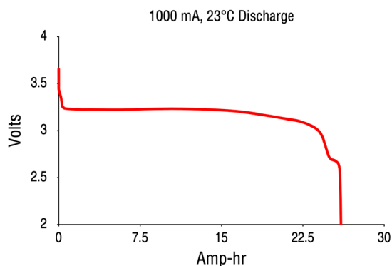
Discharge Curve 1000 mA, 23°C
