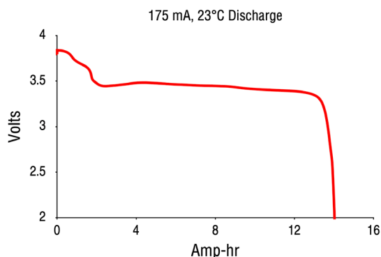
Discharge Curve 175 mA, 23°C
