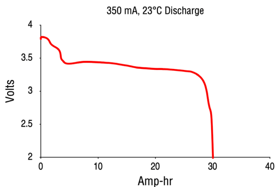
Discharge Curve 350 mA, 23°C
