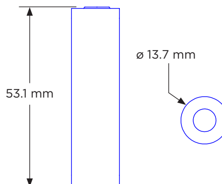
Cell Drawing
