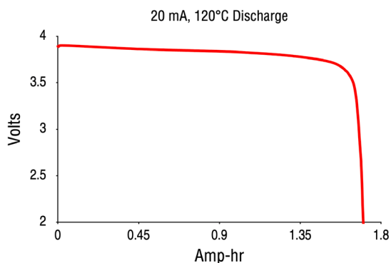
Discharge Curve 20 mA, 120°C
