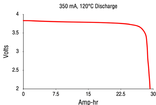
Discharge Curve 350 mA, 120°C
