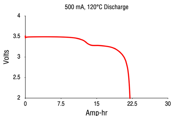
Discharge Curve 500 mA, 120°C
