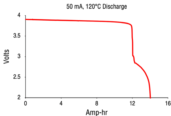
Discharge Curve 50 mA, 120°C
