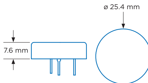
Cell Drawing
