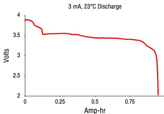
Discharge Curve 3 mA, 23°C
