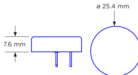
Cell Drawing
