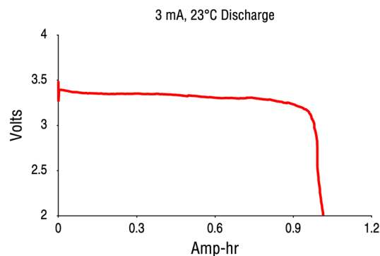
Discharge Curve 3 mA, 23°C
