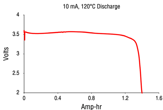
Discharge Curve 10 mA, 120°C
