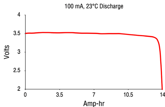
Discharge Curve 100 mA, 23°C
