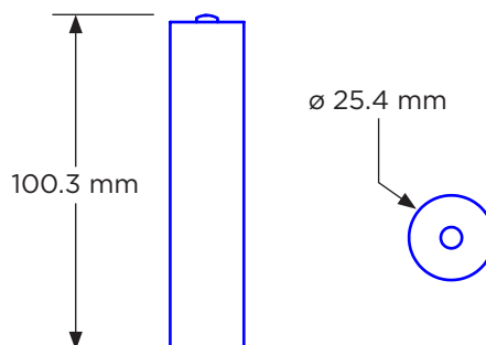
Cell Drawing
