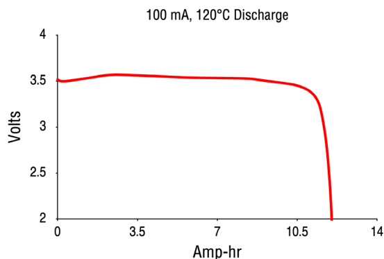
Discharge Curve 100 mA, 120°C
