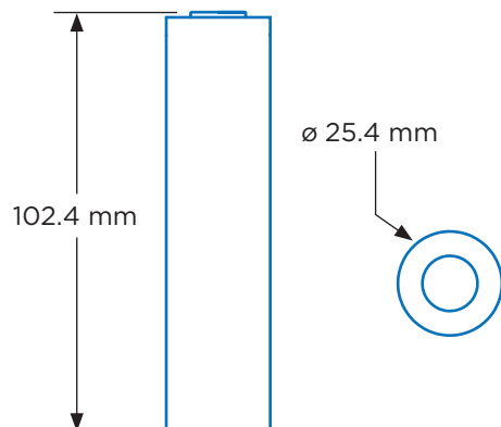
Cell Drawing
