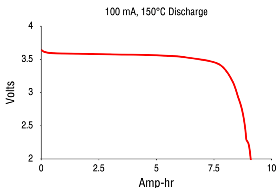
Discharge Curve 100 mA, 150°C
