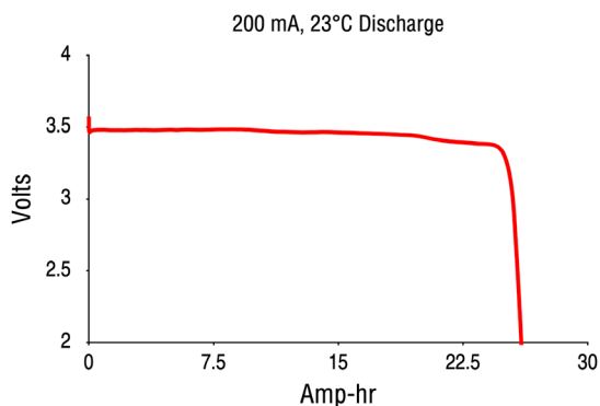
Discharge Curve 200 mA, 23°C
