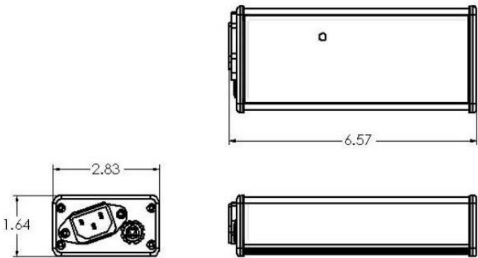
POWER ADAPTER (CH0010)
