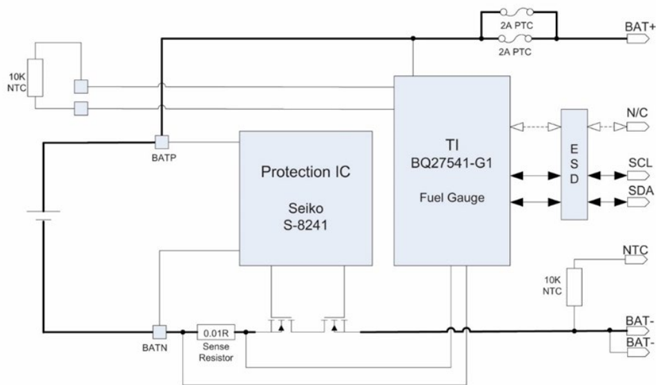
Figure 5 - Battery Electronics Block Diagram
