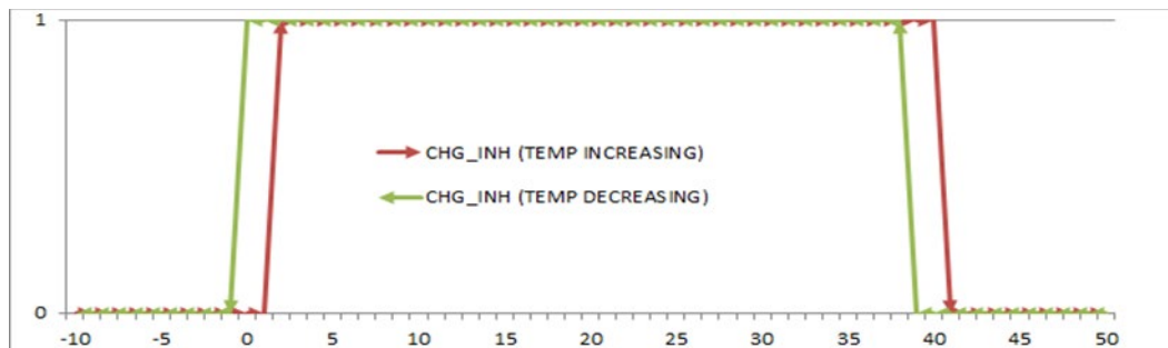
Figure 4 - CHG_INH Operation
