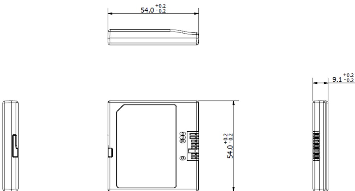
Figure 6 - Battery Dimensions
